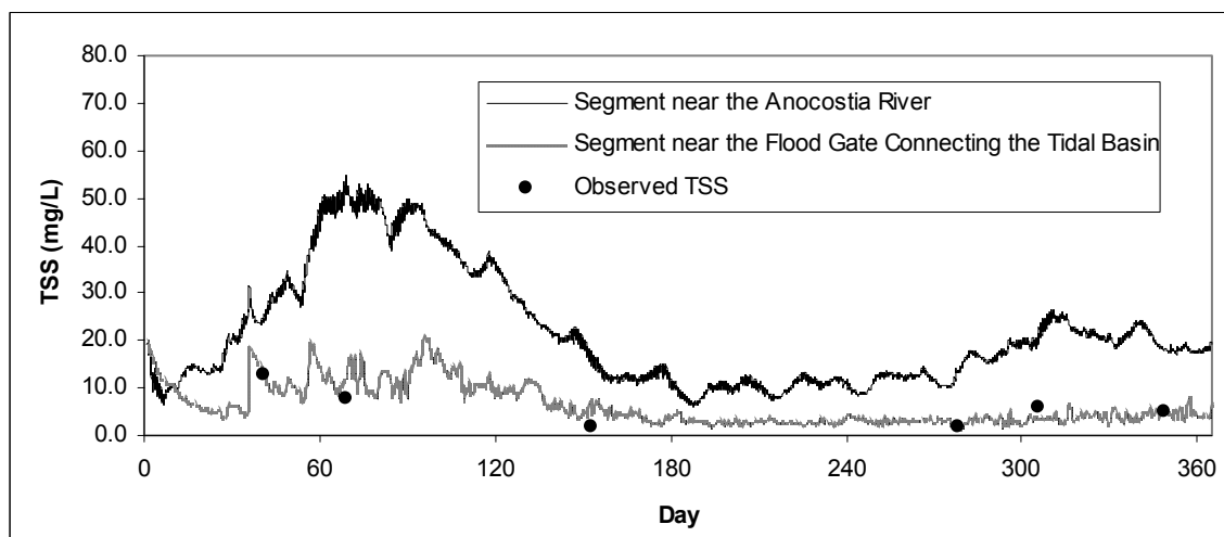
Figure 10: Modeled and Observed Suspended Solids in the Washington Ship Channel
