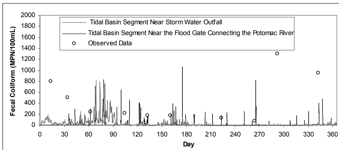
Figure 11: Modeled and Observed Fecal Coliform in the Tidal Basin for the Year 1998
