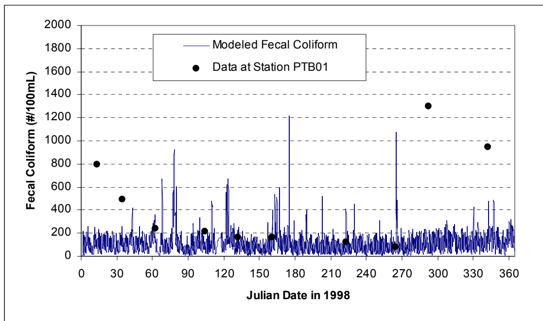
Figure 14: Modeled and Observed Fecal Coliform in the Tidal Basin for the Year 1998
